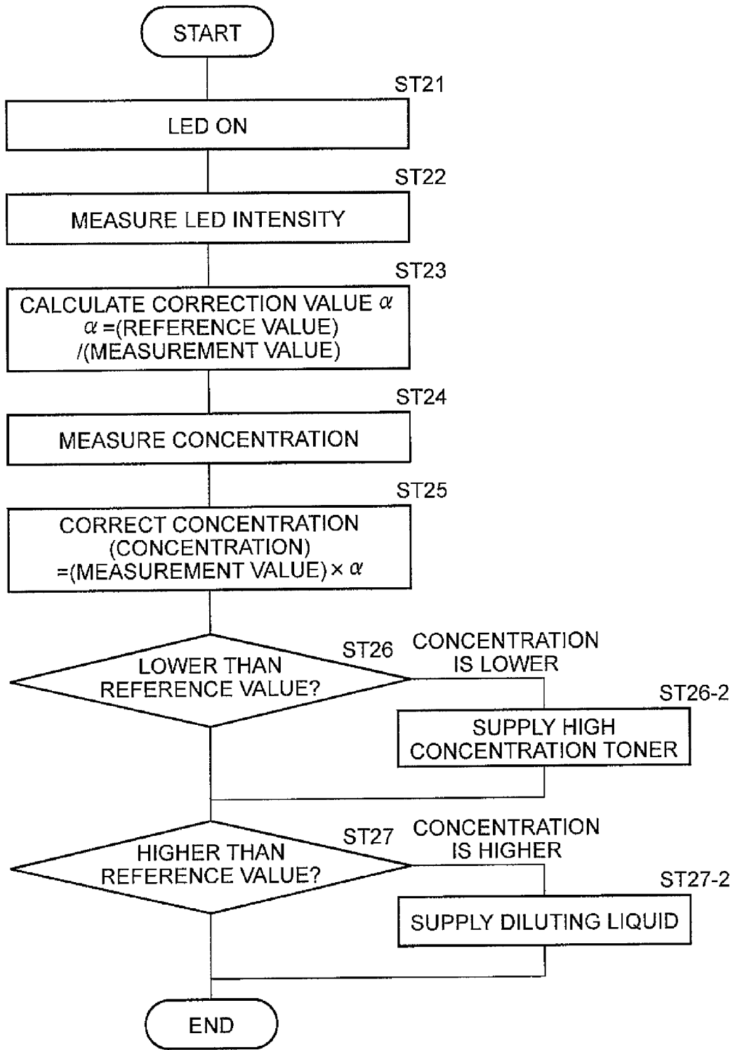
MEASUREMENT FLOWCHART
