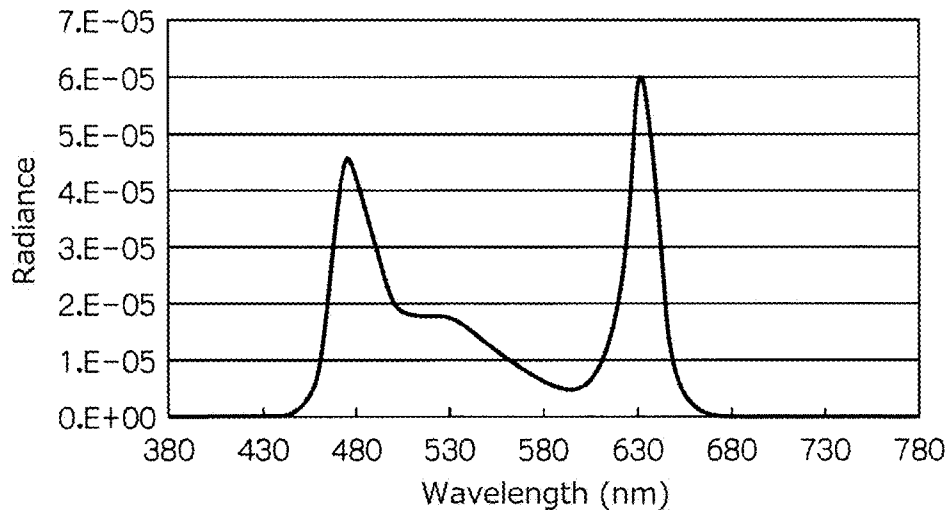
Spectral Distribution 1cd/m 2 LED5500K(new2)
