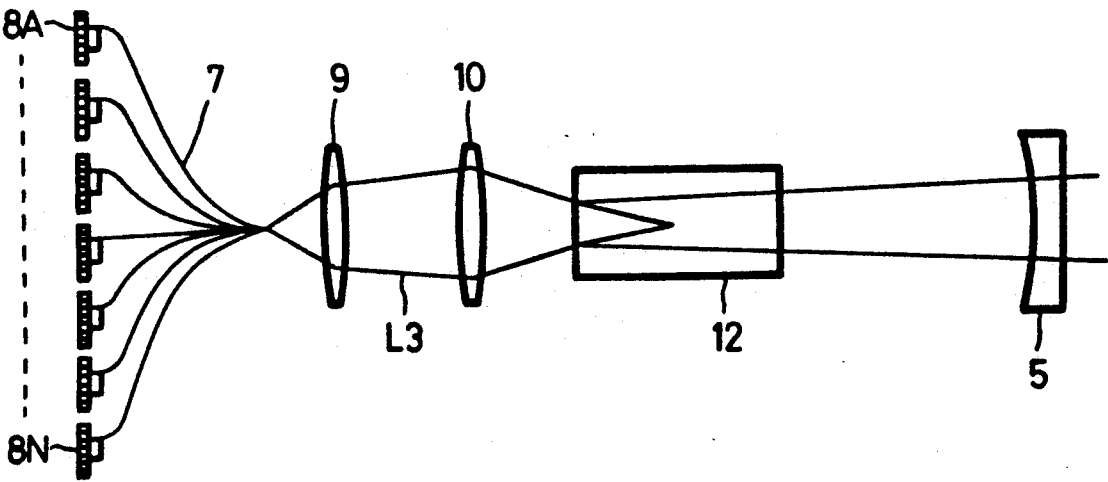
FIG. 3 PRIOR ART
