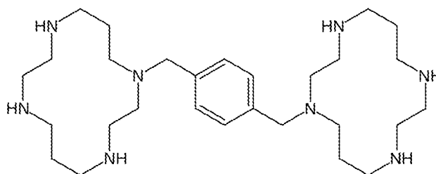
AMD3100
