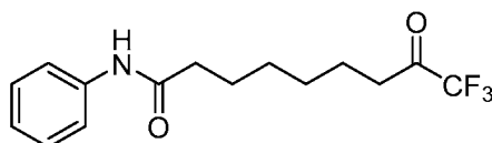
Trifluoromethyl ketone
