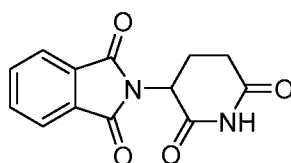
Thalidomide (racemic mixture)
