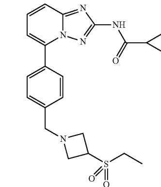
N-(5-(4-((3-(ethylsulfonyl)azetidin-1-yl)methyl)phenyl)-[1,2,4]triazolo[1,5-a]pyridin-2-yl)cyclopropanecarboxamide
