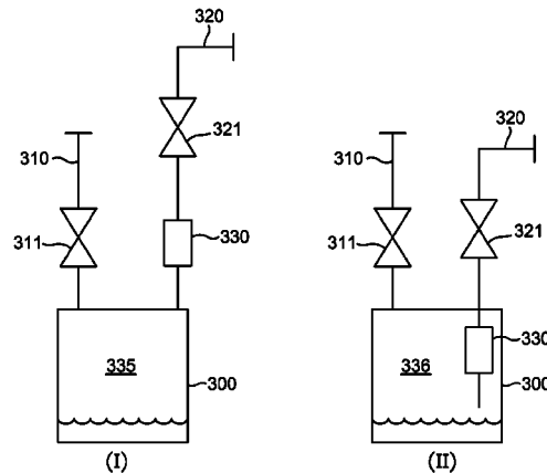
Package for Sb containing dopant materials
