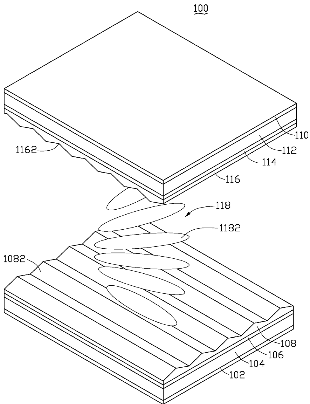
FIG. 4 (RELATED ART)
