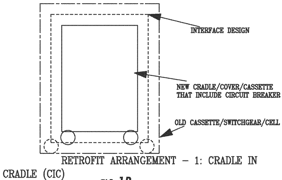
RETROFIT ARRANGEMENT - 1: CRADLE IN CRADLE (CIC)
