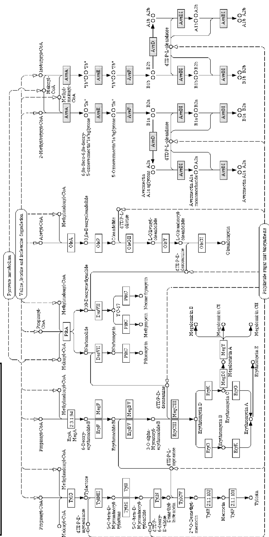
BIOSYNTHESIS OF 12-, 14- AND 16-MEMBERED MACROLIDES
