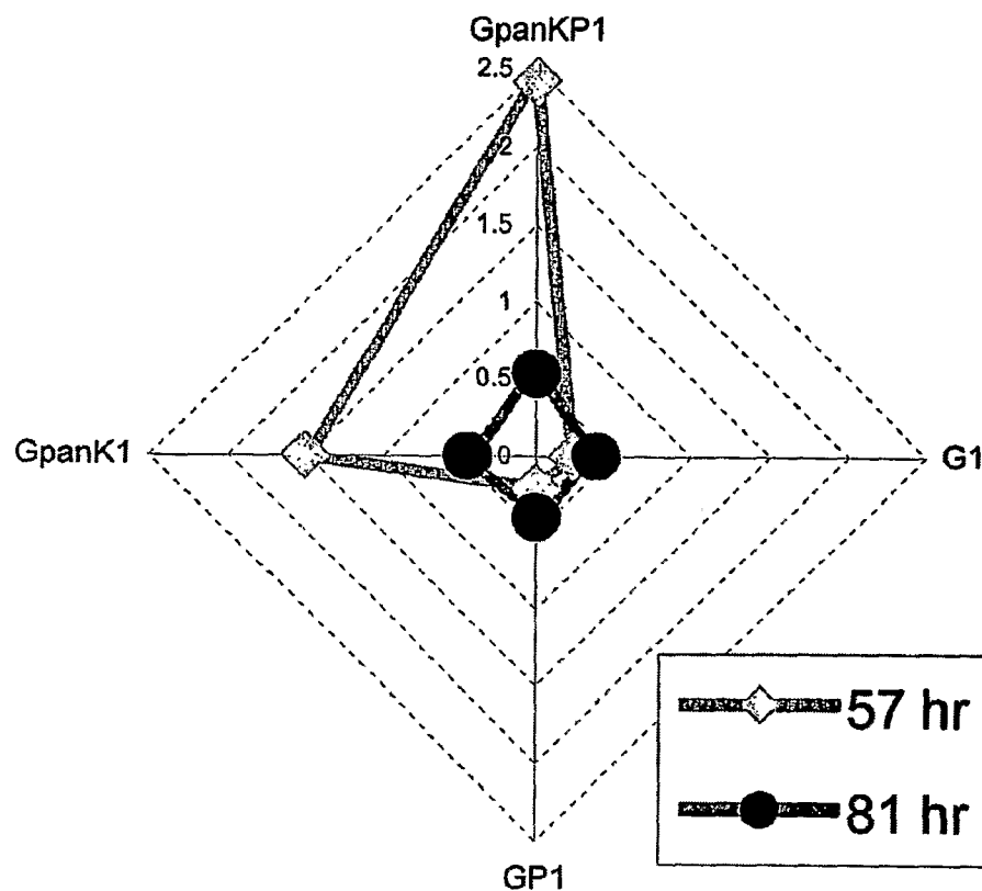
FIG. 4. Deoxyoleandolide production
