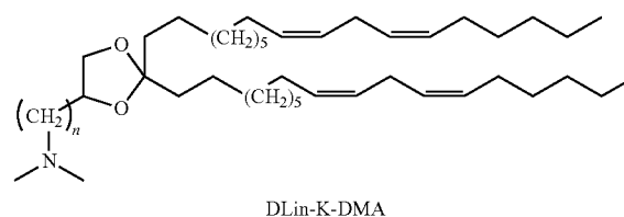
DLin-K-DMA
