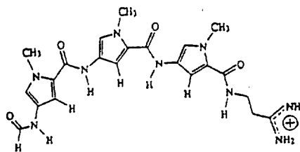
Distamycin A (Dst)
