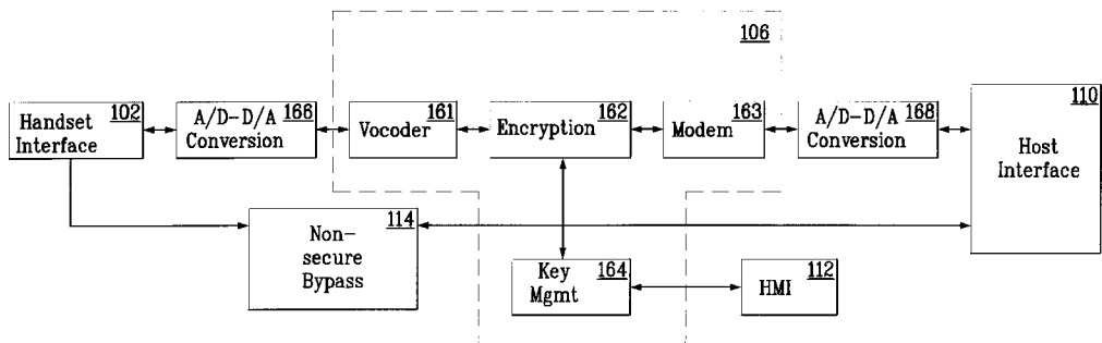
SCS Functional Block Diagram
