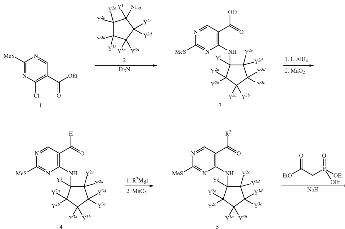
Scheme I. Synthesis of Compounds of Formula I wherein Z is hydrogen.
