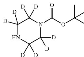
Scheme 4: Analogs of Intermediate 13
