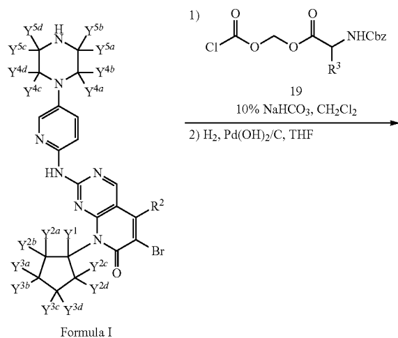
Scheme 6. Synthesis of Compounds of Formula I wherein Z is -\text{C}(\text{O})\text{OCH}_2\text{OC}(\text{O})\text{CH}(\text{R}^3)\text{NH}_2 .
