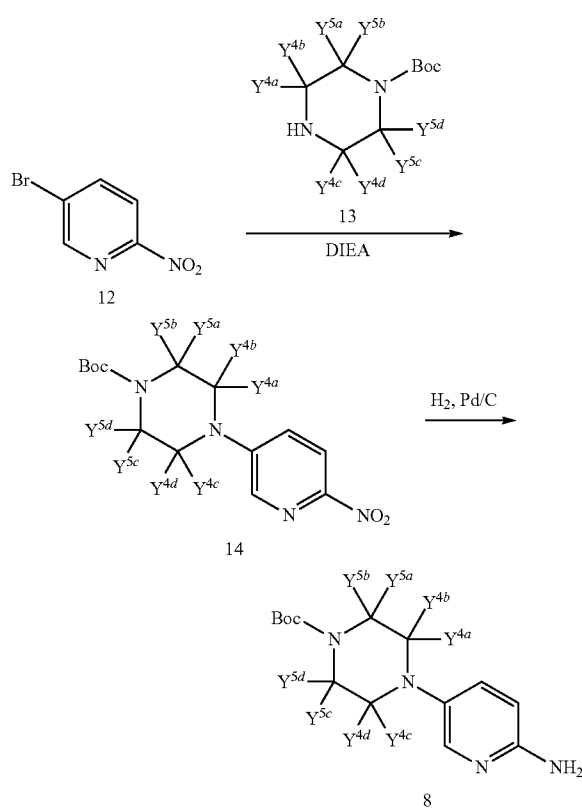
Scheme 3: Synthesis of Intermediate 8
