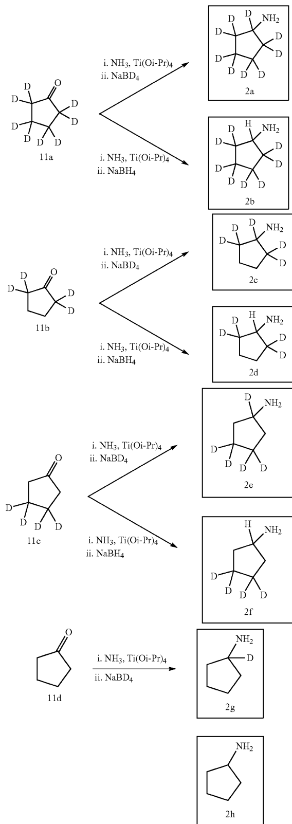
Scheme 2: Access to Analogs of Intermediate 2
