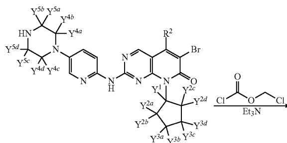
Scheme 5b. Alternative Synthesis of Compounds of Formula I wherein Z is -\text{C}(\text{O})\text{OCH}_2\text{OP}(\text{O})(\text{OH})_2 .
