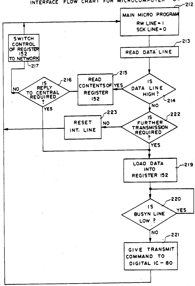
FIG. 15 INTERFACE FLOW CHART FOR MICROCOMPUTER - 84
