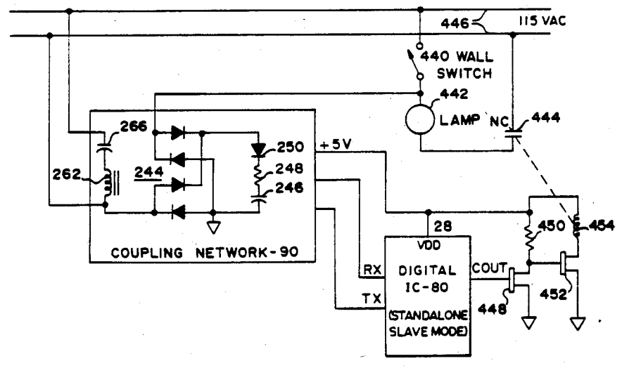
FIG. 39 LOCAL OVERRIDE CIRCUIT
