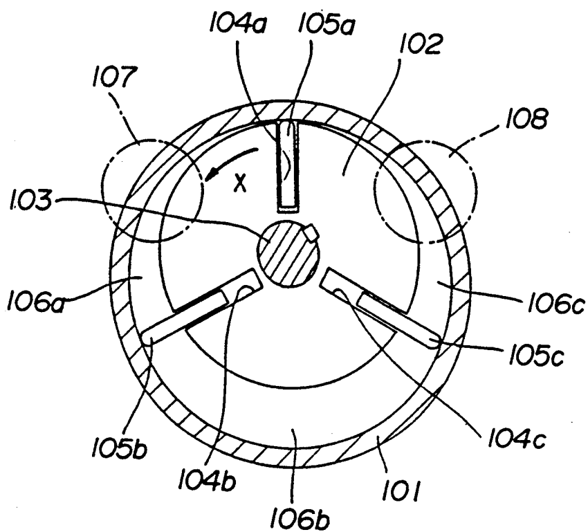
FIG. 12 PRIOR ART
