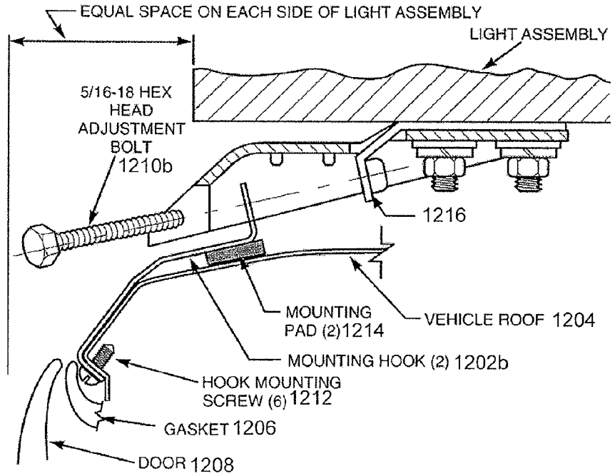
FIG. 5B (Hook mount for vehicles without gutter.)
