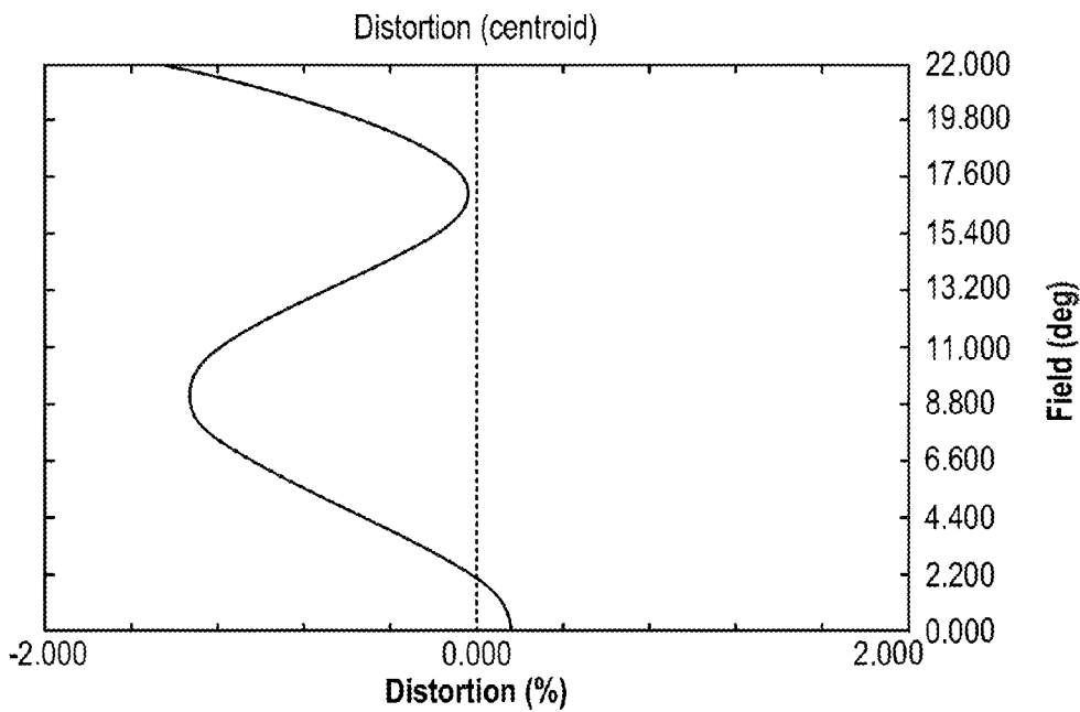
30/06/2013 Maximum distortion = 1.5%
