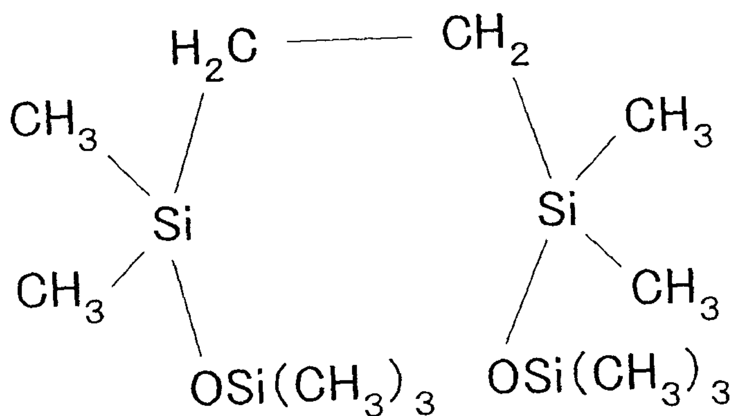
[CHEMICAL FORMULA 4]
