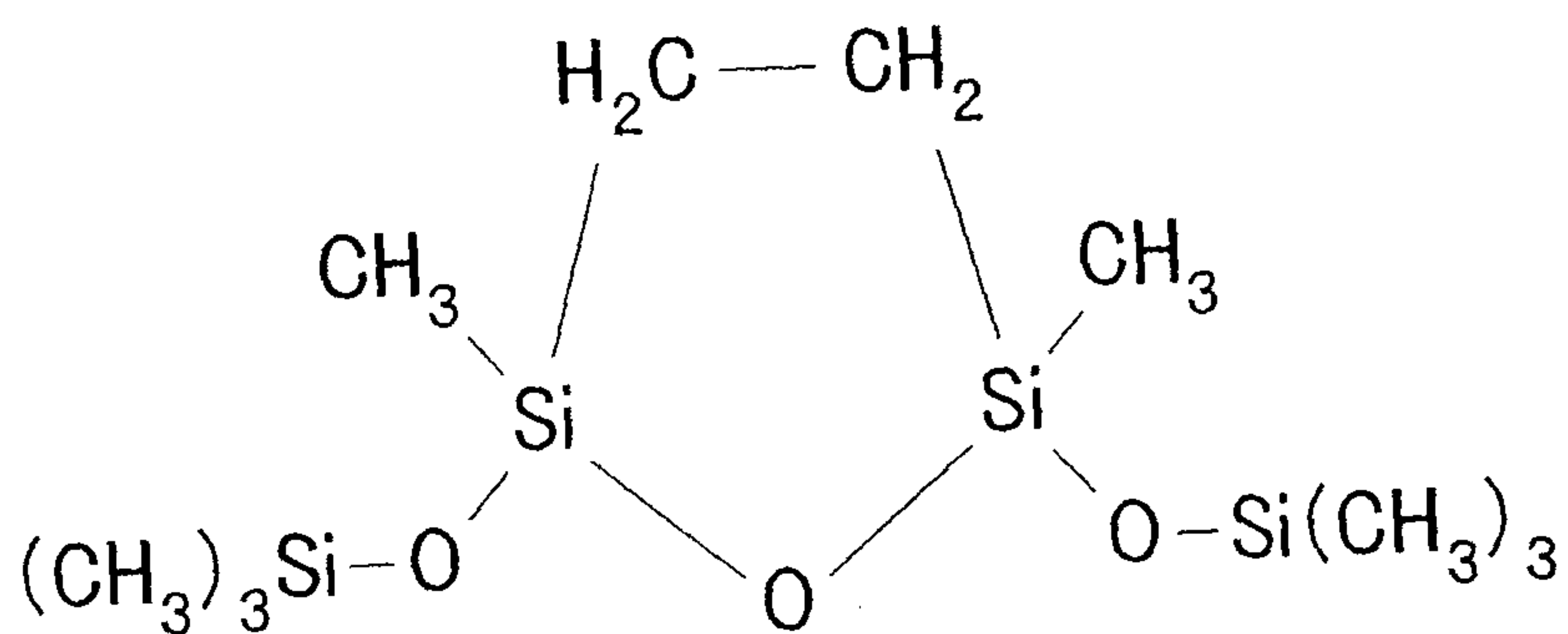
[CHEMICAL FORMULA 2]
