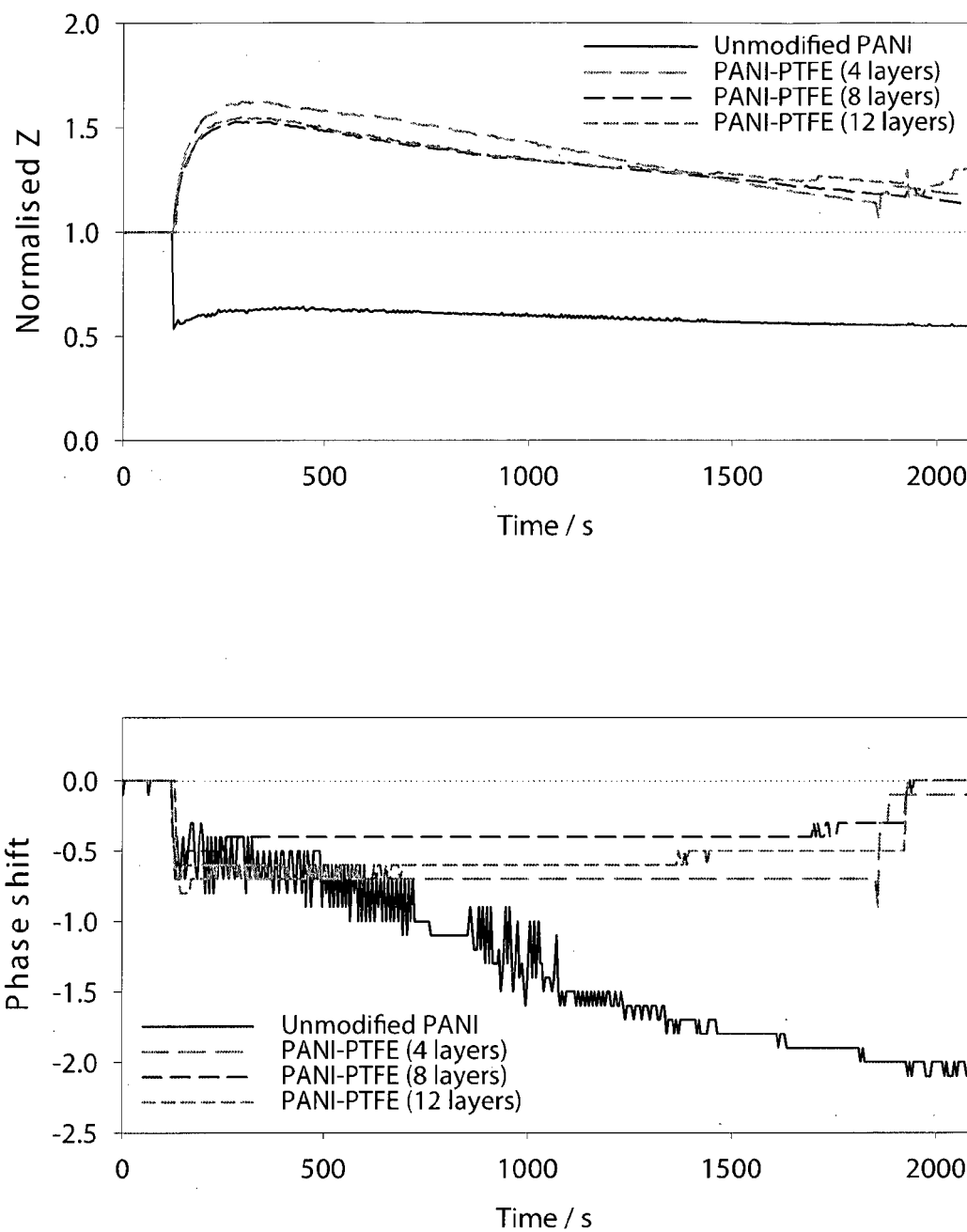
Figure 28. Impedance time plots displaying the effect of 50ppm ammonia on PANI films modified with different print thicknesses of PTFE particles.
