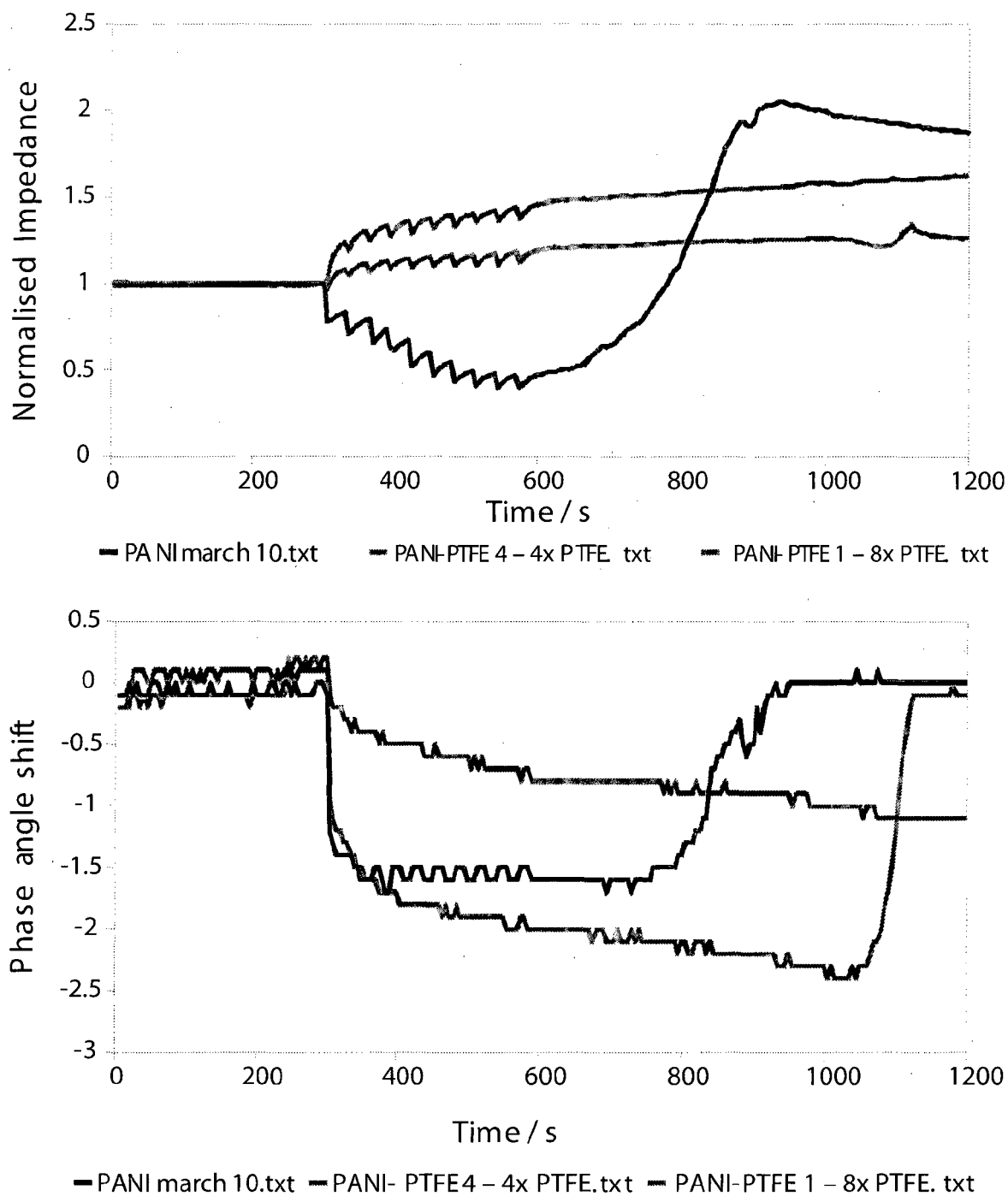
Figure 31a. Response of PTFE -modified (10 \mu\text{m} resolution of 4 and 8 layers) and Figure 31b Response of an unmodified PANI sensor to. Ten exhales performed starting at 300s and at 30s intervals thereafter. a) Impedance-time and b) phase angle-time.
