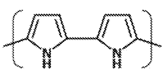
\alpha, \alpha'
