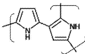
\alpha, \beta'
