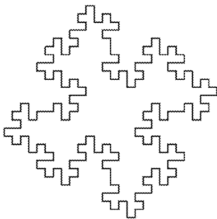
(a) Fractal Curve
