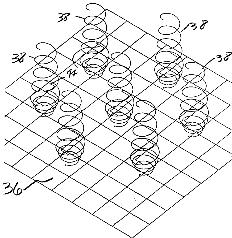
Cluster of seven dual port helices
