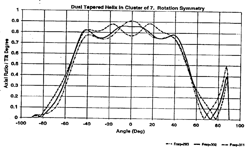
Fig. 15 Axial ratio of dual port helix: dipole excitation
