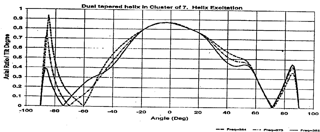
Fig. 12 Axial ratio of dual port helix: helix excitation
