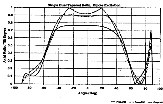
Fig. 5 Axial ratio of dual port helix: dipole excitation
