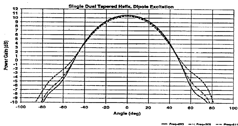
Fig. 4 Pattern diagram of dual port helix: dipole excitation
