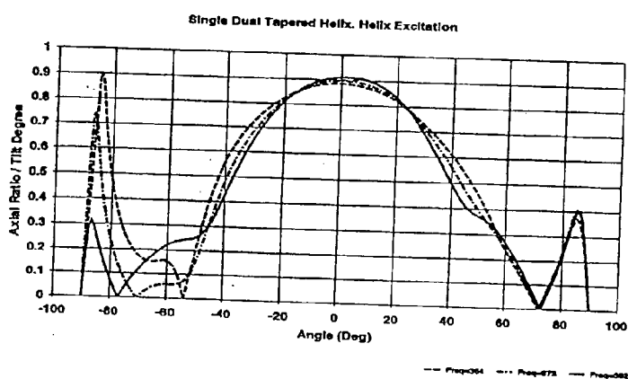
Fig. 7 Axial ratio of dual port helix: helix excitation
