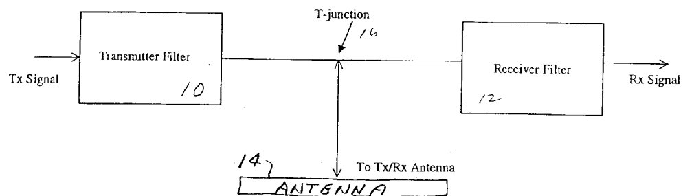
Figure 1A Equivalent circuit of multifold diplexer. (PRIOR ART)
