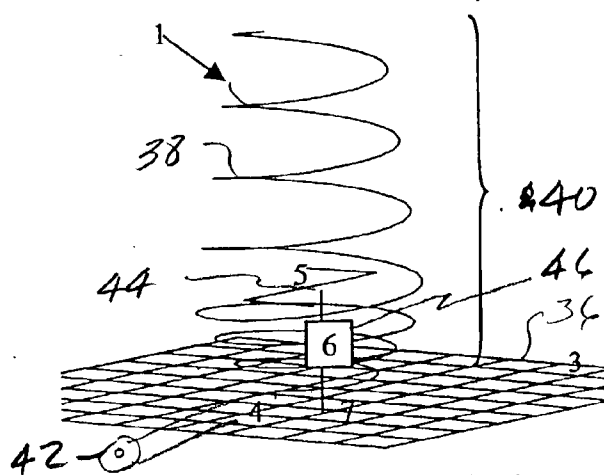
Fig. 3 Helix with Z-shaped dipole
