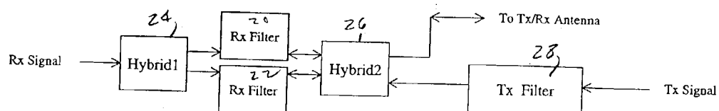
Figure 1B Equivalent circuit of directional filter multiplexer (PRIOR ART)
