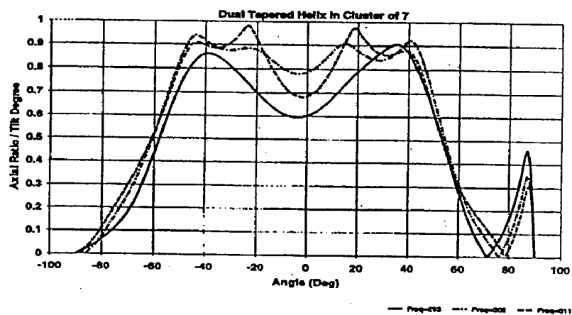
Fig. 10 Axial ratio of dual port helix: dipole excitation
