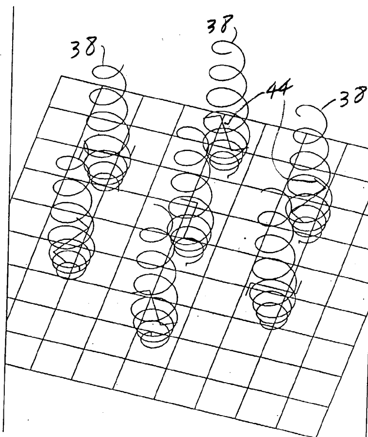
Fig. 13 Cluster of seven dual port helices with rotation symmetry
