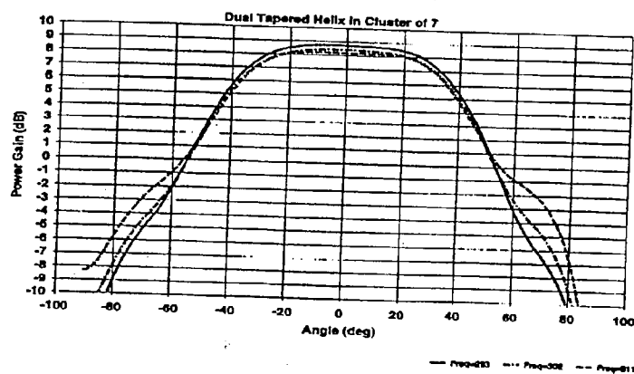
Fig. 9 Pattern diagram of dual port helix: dipole excitation
