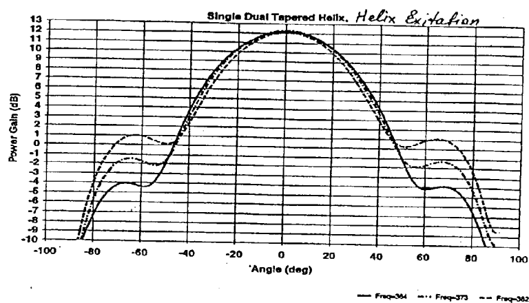
Fig. 6 Pattern diagram of dual port helix: helix excitation
