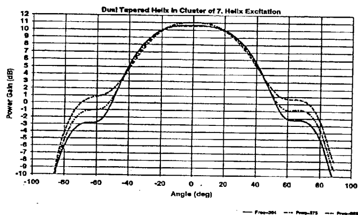
Fig. 11 Pattern diagram of dual port helix: helix excitation
