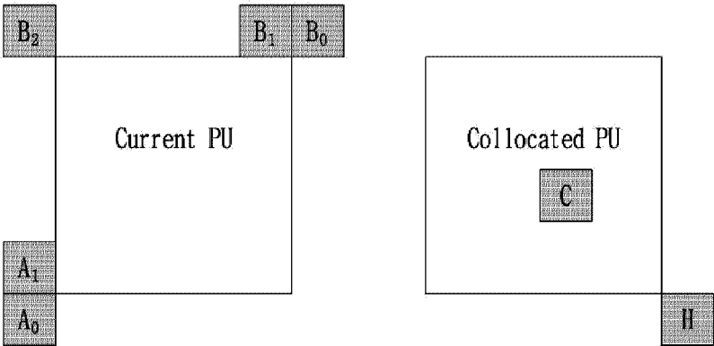
(a) temporally/spatially adjacent block of AMVP
