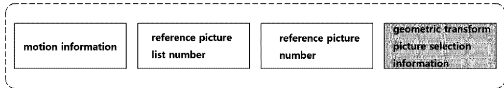
(b) example of inter prediction information construction of encoder/decoder using geometric transform picture
