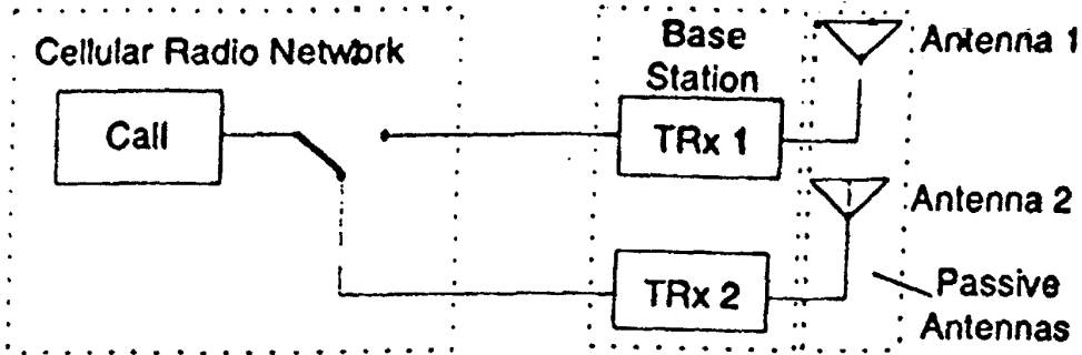
Fig. 4 (a) Conventional Cellular System
