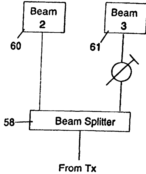
Fig. 14 (b) Quadrature
