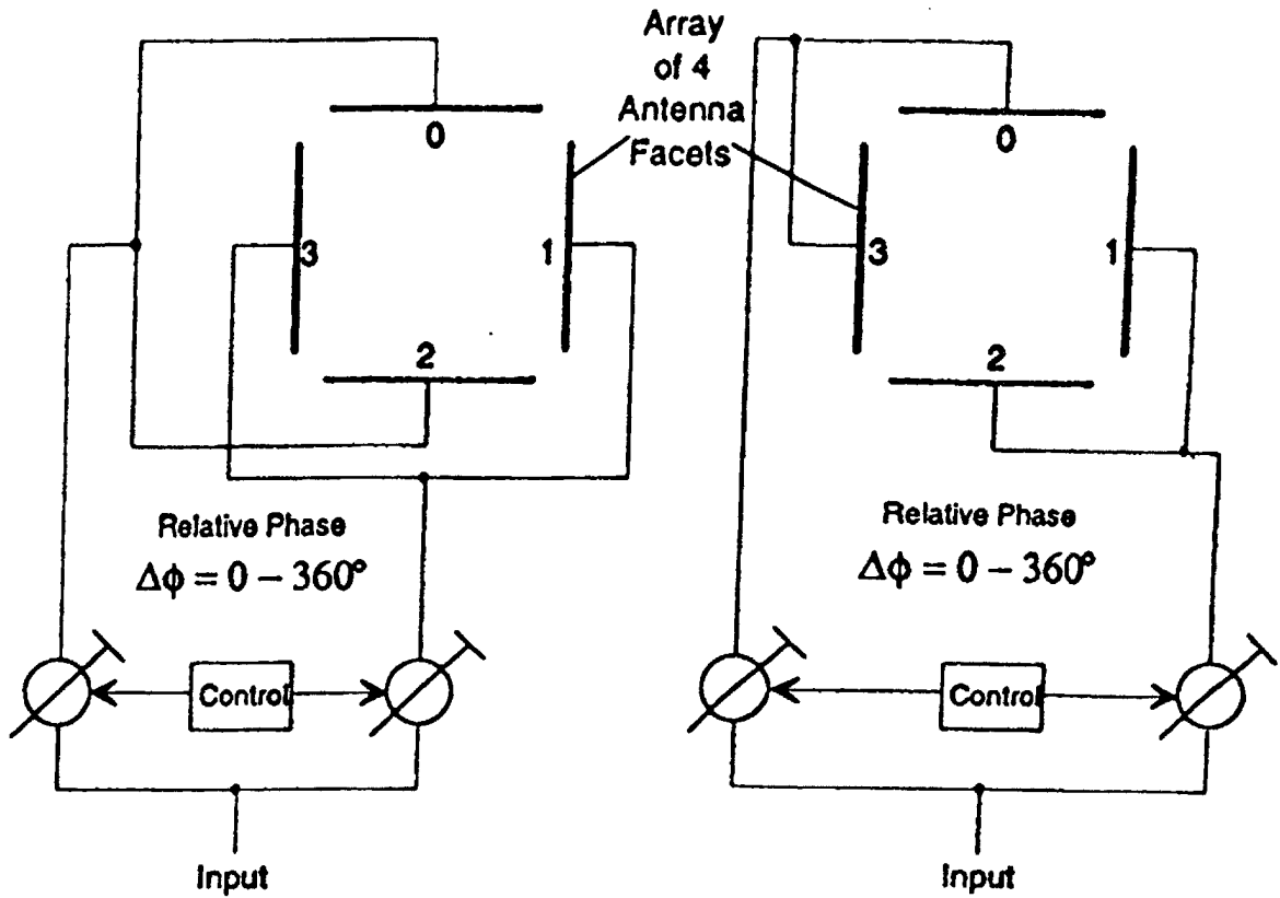
Fig. 12 (a) Preferred Embodiment
