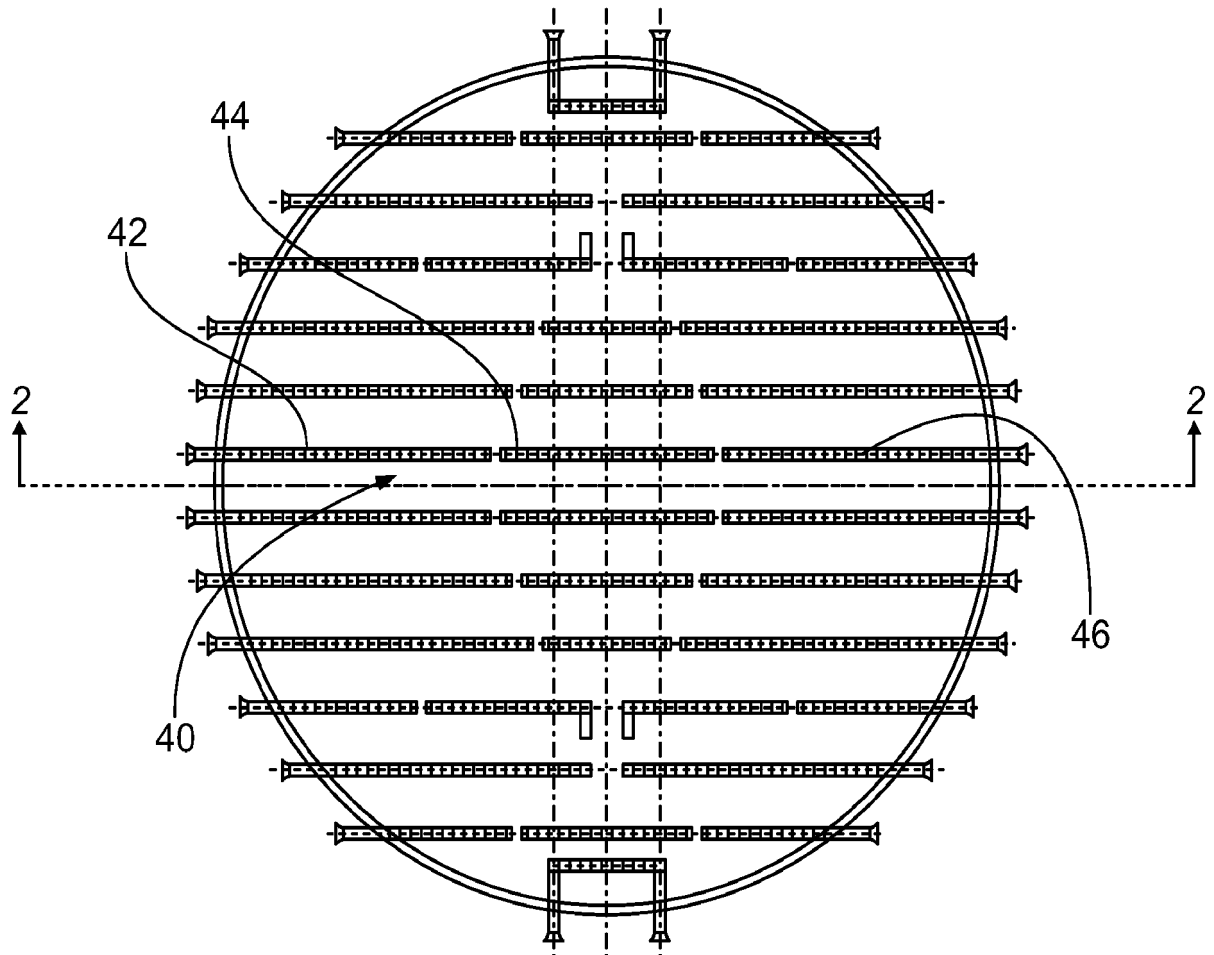
FIG. 3 (PRIOR ART)
