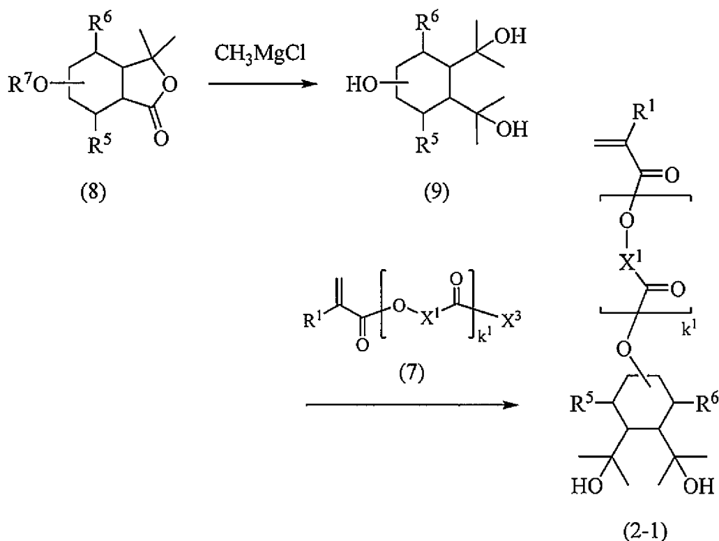
Scheme B
