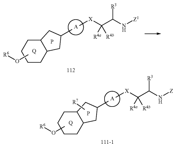
<Reaction Scheme 43>
