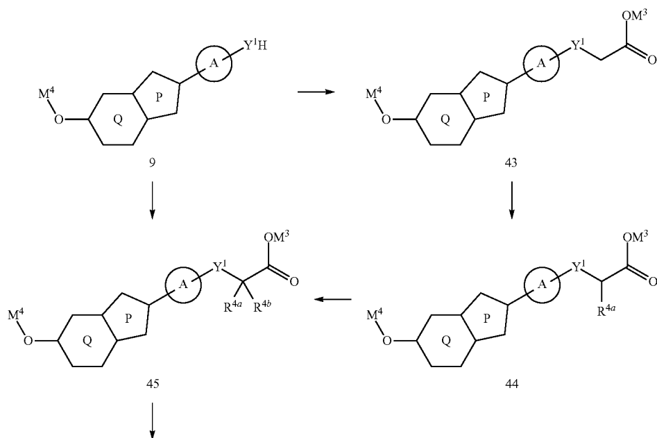
<Reaction Scheme 16>
