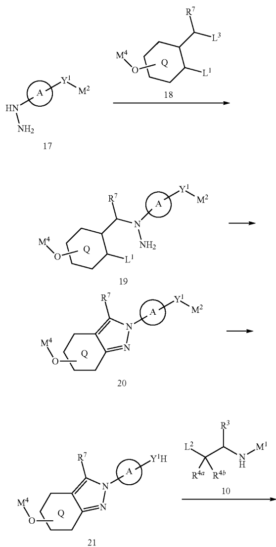
Reaction Scheme 6
