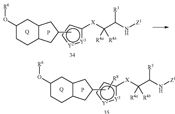
Reaction Scheme 10
