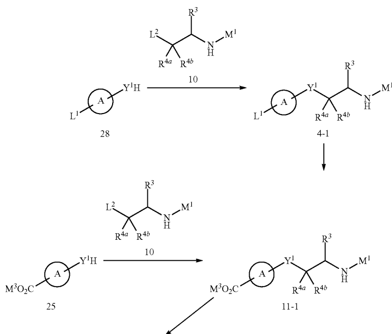
<Reaction Scheme 7>
