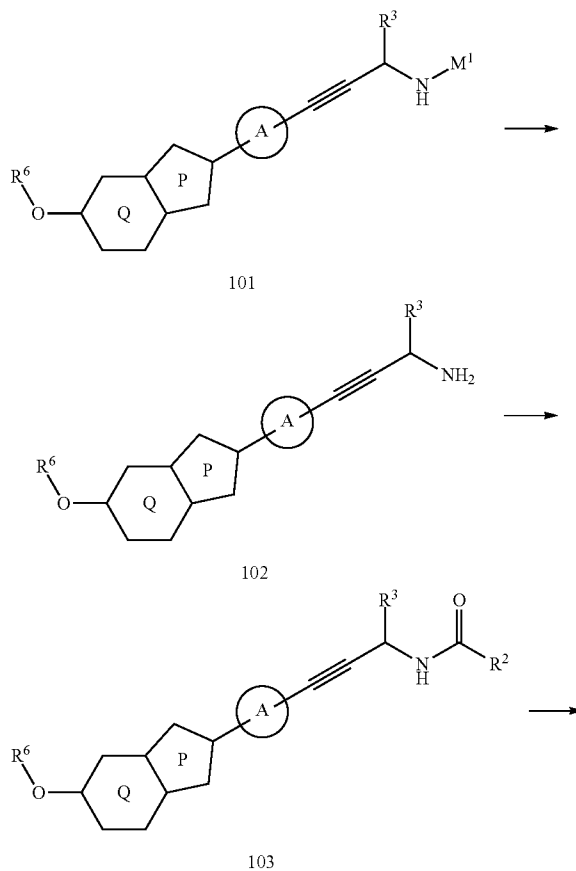
<Reaction Scheme 30>
