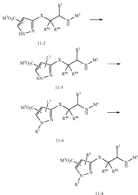
<Reaction Scheme 27>
