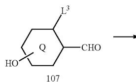
<Reaction Scheme 34>
