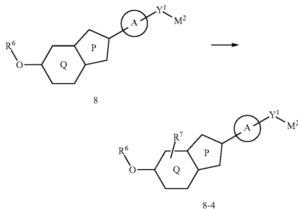
<Reaction Scheme 37>
