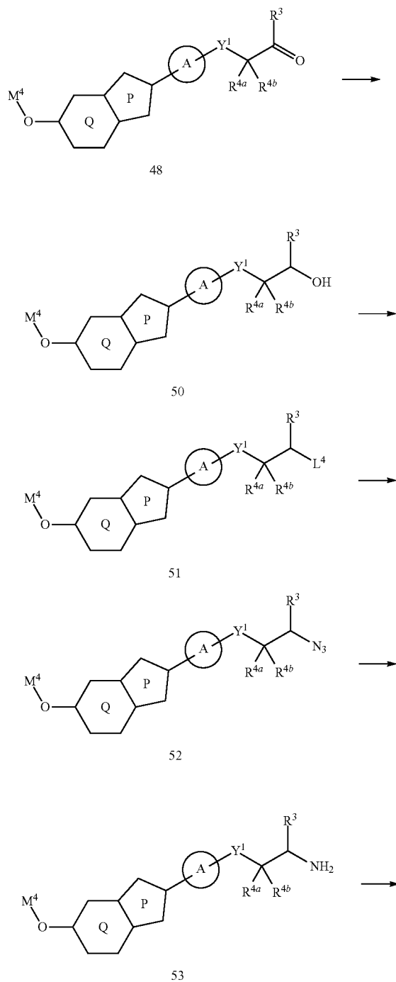
<Reaction Scheme 17>
