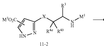
Reaction Scheme 9
