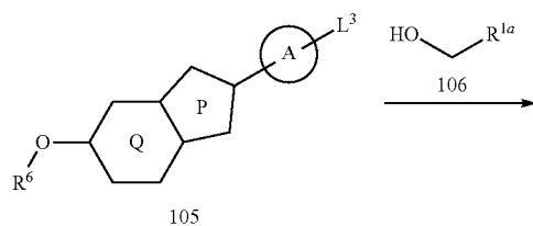
<Reaction Scheme 33>
