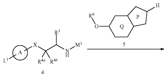
Reaction Scheme 3
