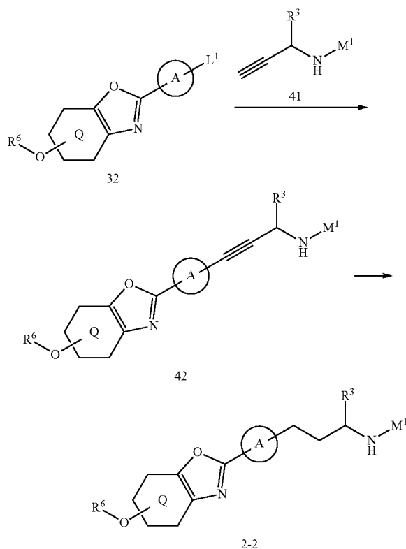
<Reaction Scheme 15>
