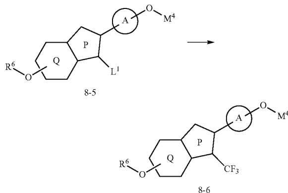
<Reaction Scheme 38>
