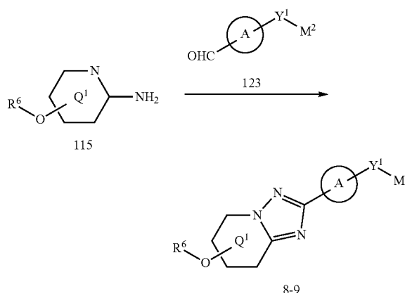
<Reaction Scheme 44>
