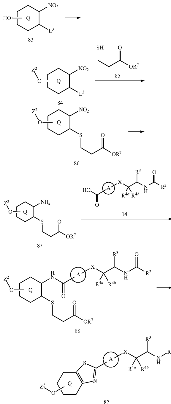
<Reaction Scheme 26>
