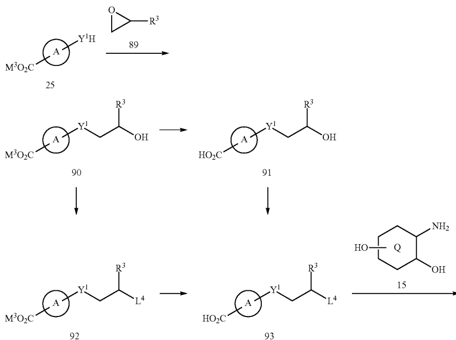
<Reaction Scheme 28>
