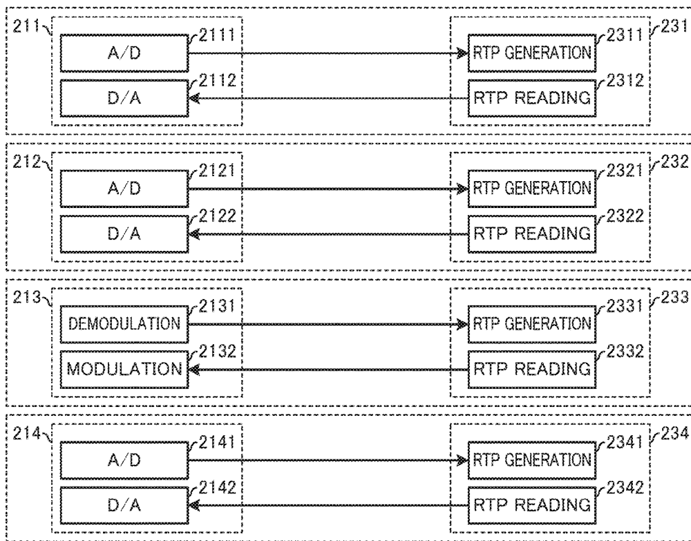
(A) :AUDIO SIGNAL
