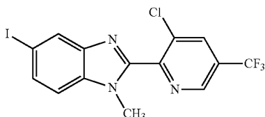
Intermediate Compound (M6-41)
