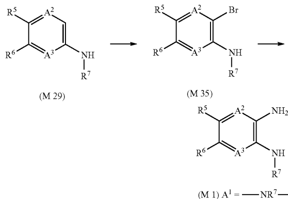
(M 1) A 1 = —NR 7 —
