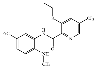
Intermediate Compound (M3-32)
