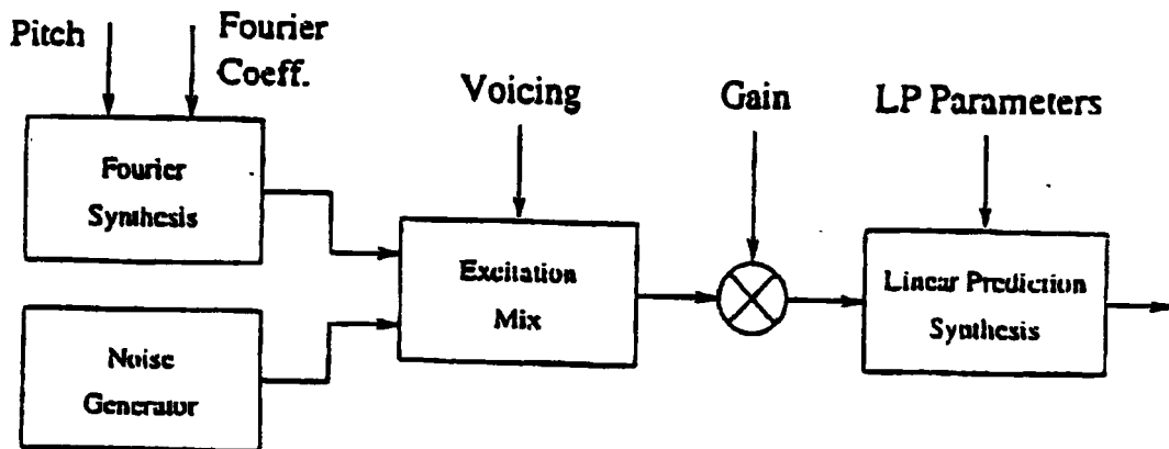
Figure 2b MELP synthesis
