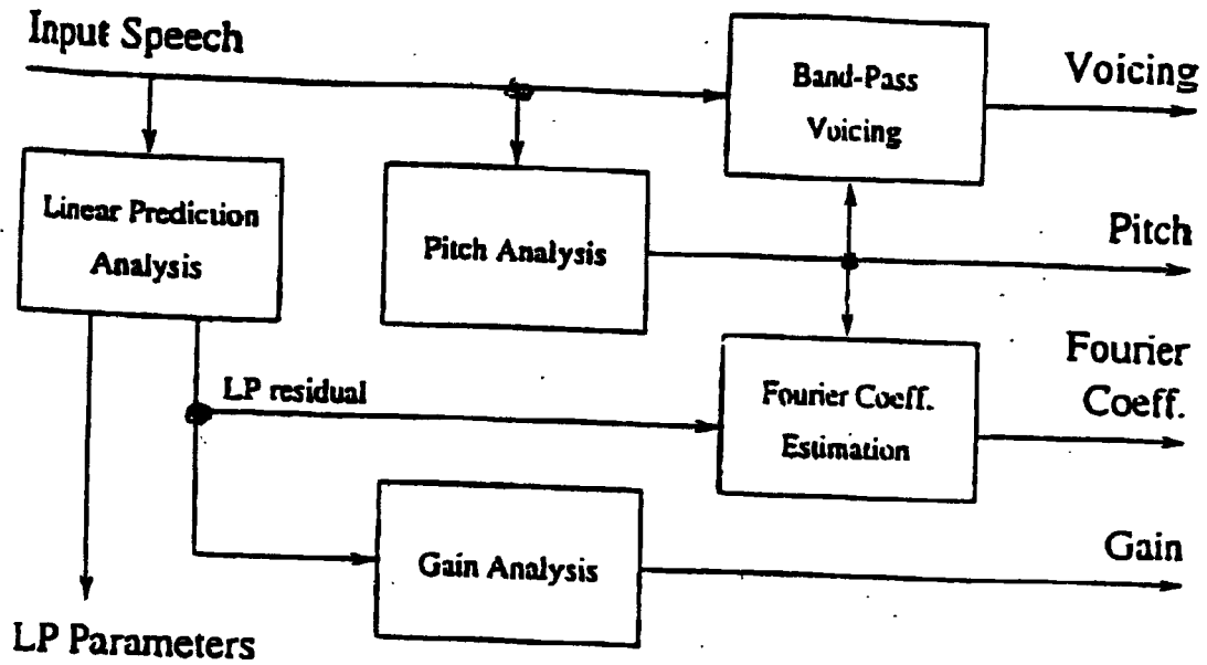
Figure 1a MELP analysis
