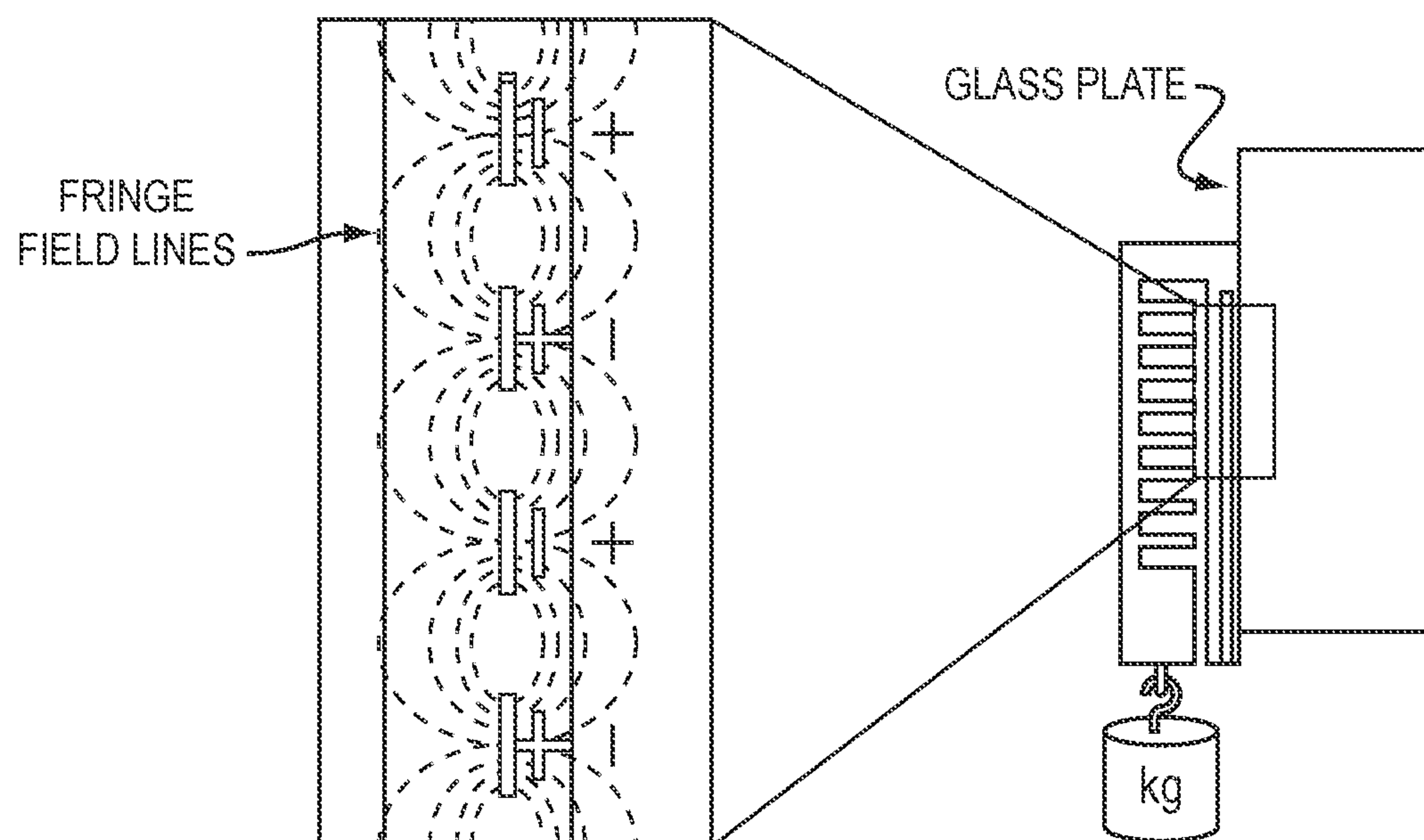
FIG. 29C SOFT ACTUATOR ADHERED TO A GLASS PLATE
