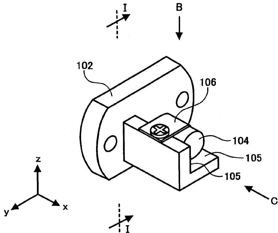
FIG. 15 (PRIOR ART)
