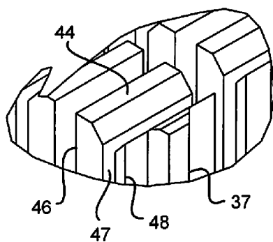
FIGURE 6C
