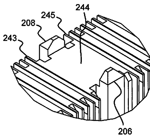
FIGURE 12D
