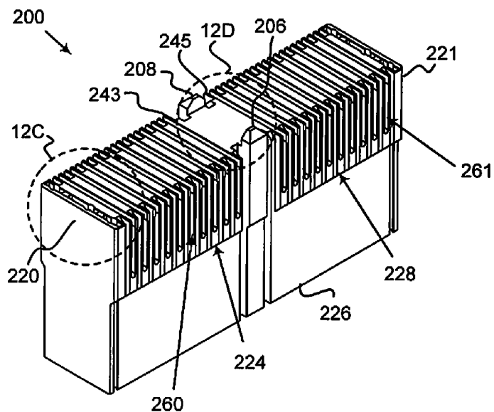
FIGURE 12A
