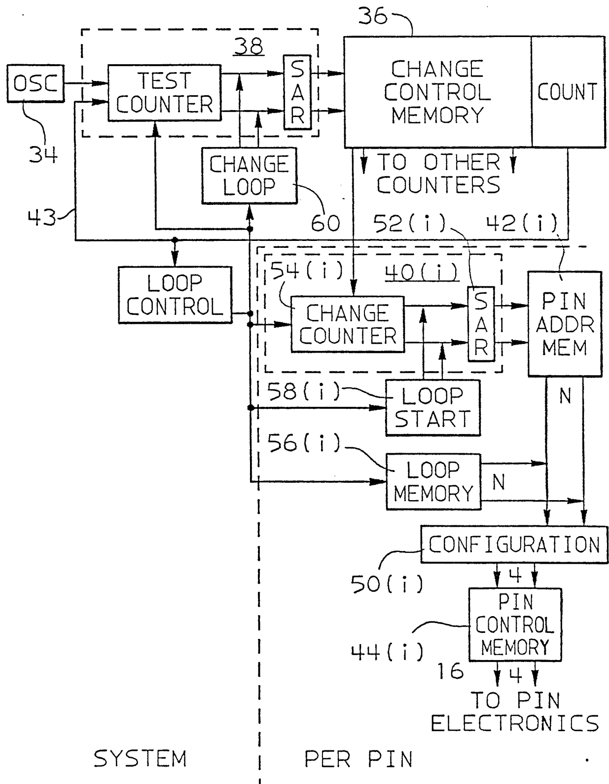
FIG. 3 HIERARCHICAL TEST SYSTEM
