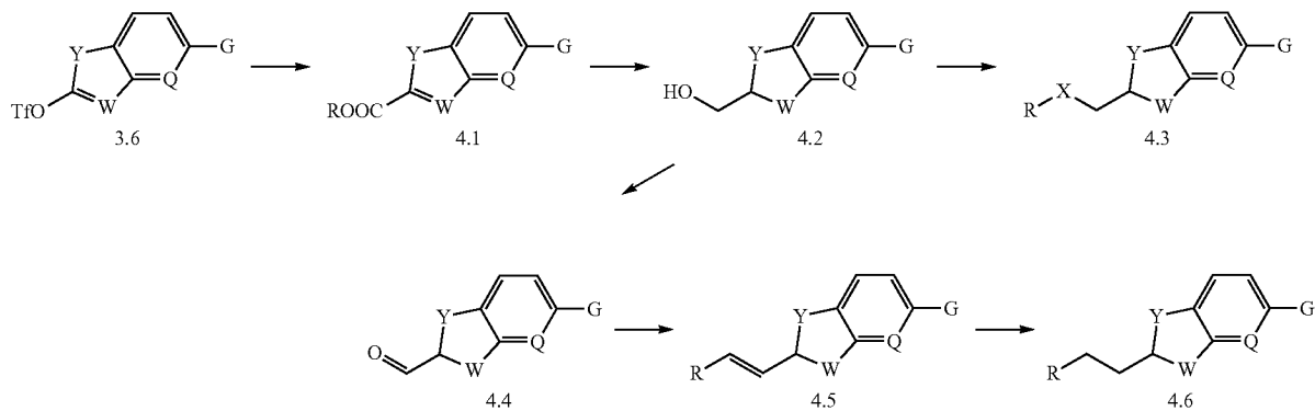
SCHEME 4
