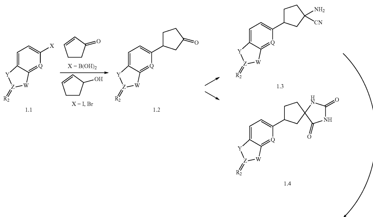
SCHEME 1
