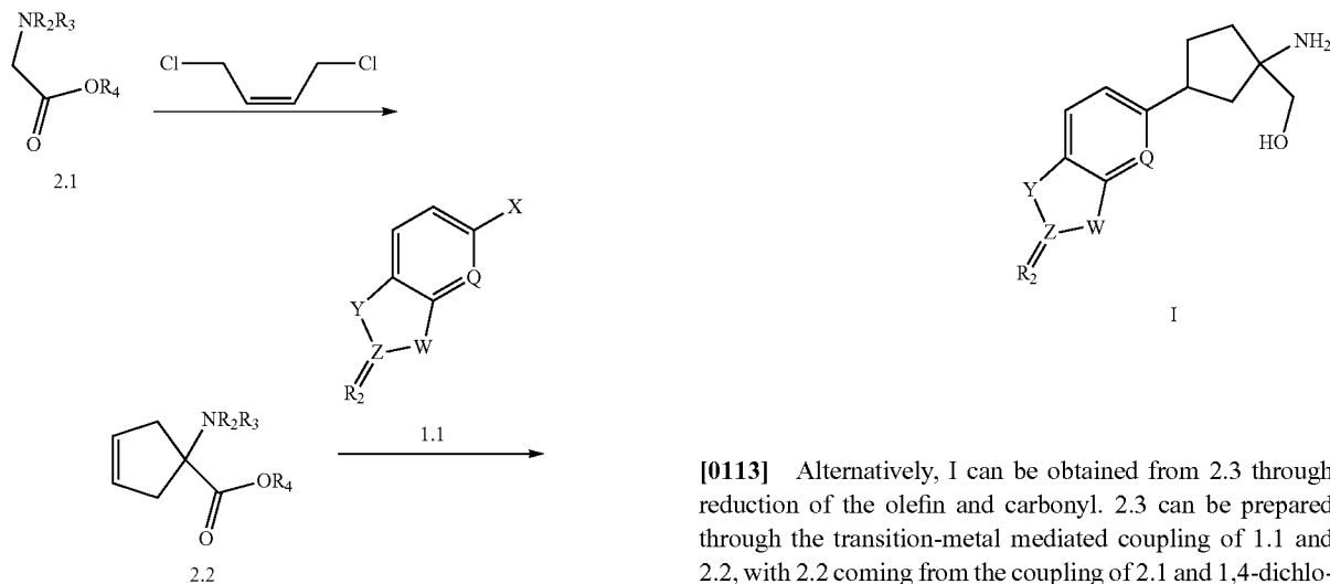
SCHEME 2
