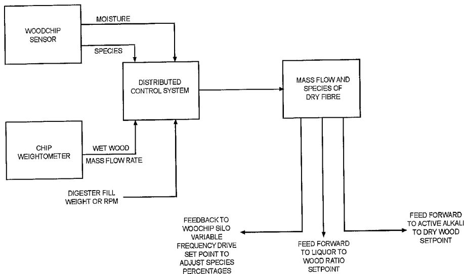
Sensor and Control System Schematic
