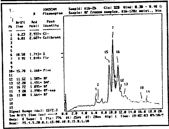
Characteristic Signature of Balsam Fir Under Different Moisture Content
