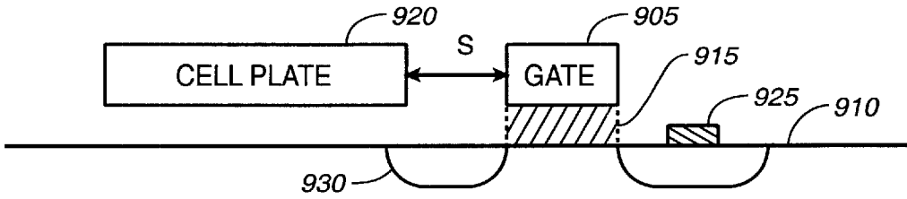
FIG. 9 (PRIOR ART)
