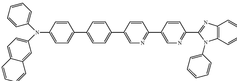
N-phenyl-N-(4'-(6'-(1-phenyl-1H-benzo[d]imidazol-2-yl)-[2,3'-bipyridin]-5-yl)-[1,1'-biphenyl]-4-yl)naphthalen-2-amine,
