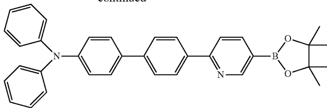
Compound 15
