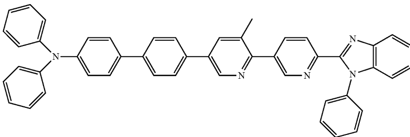
4'-(3-methyl-6'-(1-phenyl-1H-benzo[d]imidazol-2-yl)-[2,3'-bipyridin]-5-yl)-N,N-diphenyl-[1,1'-biphenyl]-4-amine,
