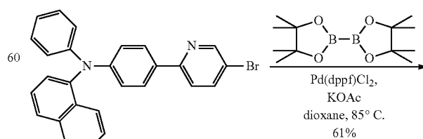
Compound 30
