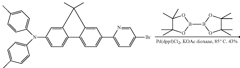
Compound 34
