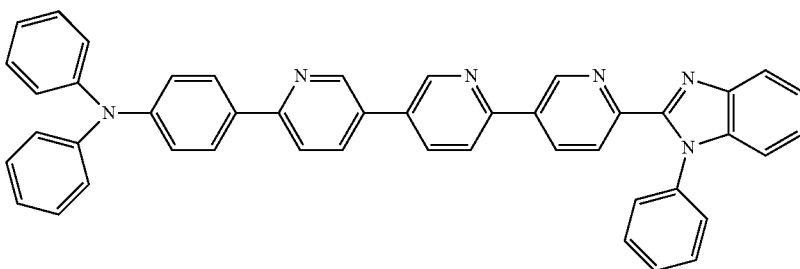
N,N-diphenyl-4-(6-(1-phenyl-1H-benzo[d]imidazol-2-yl)-[3,2':5',3''-terpyridin]-6''-yl)aniline,
