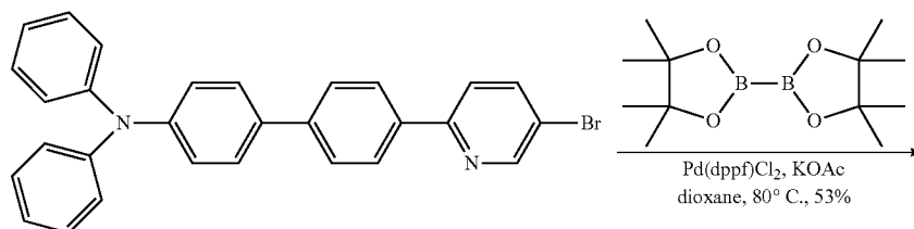
Compound 14
