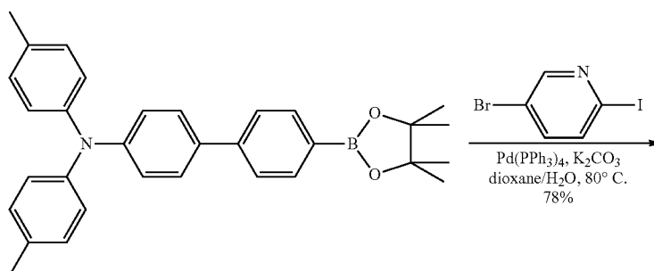
Compound 3
