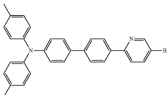
Compound 6 Molecular Weight: 475.43
