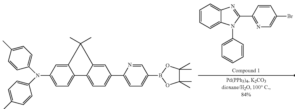
Compound 35
