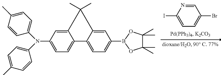
Compound 33
