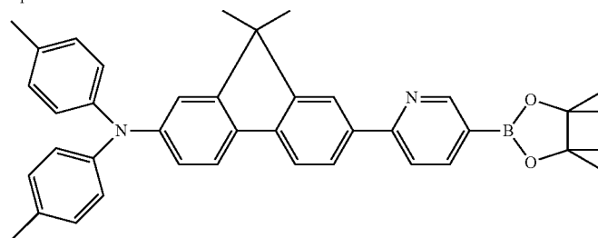
Compound 35
