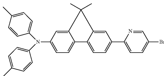
Compound 34
