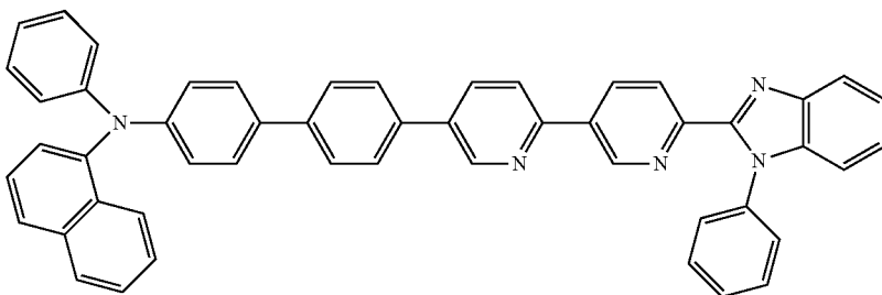
N-phenyl-N-(4'-(6'-(1-phenyl-1H-benzo[d]imidazol-2-yl)-[2,3'-bipyridin]-5-yl)-[1,1'-biphenyl]-4-yl)naphthalen-1-amine,
