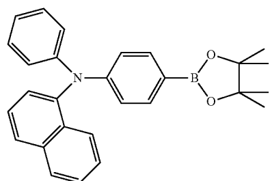
Compound 29
