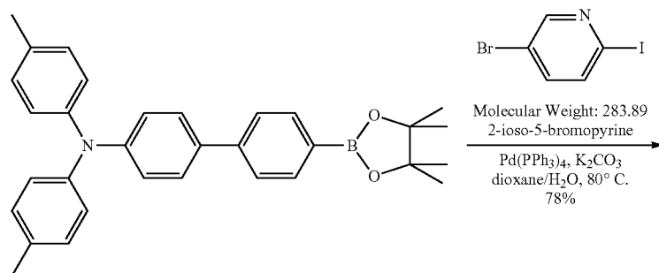
Compound 3
