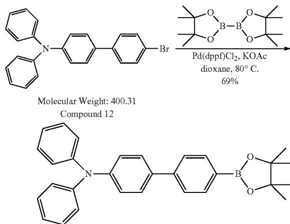
Compound 13
