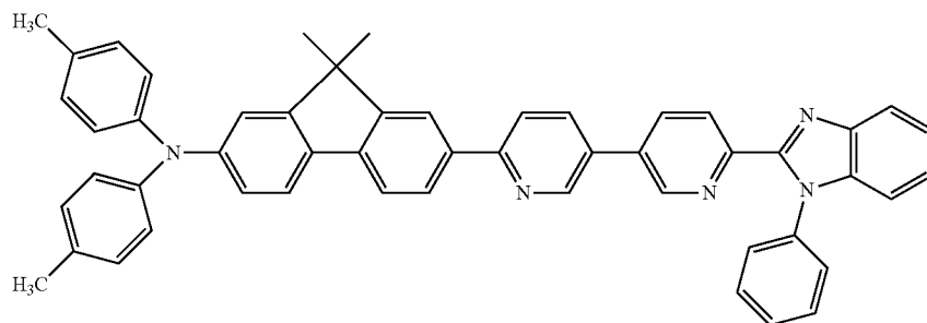
9,9-dimethyl-7-(6'-(1-phenyl-1H-benzo[d]imidazol-2-yl)-[3,3'-bipyridin]-6-yl)-N,N-di- p -tolyl-9H-fluoren-2-amine
