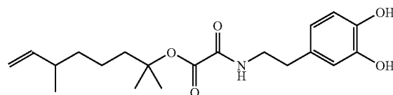
BF-compound 39
