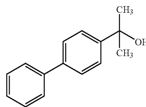
2-(4-biphenyl)-propan-2-ol
