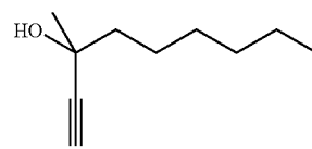
3-methyl-1-nonyn-3-ol
