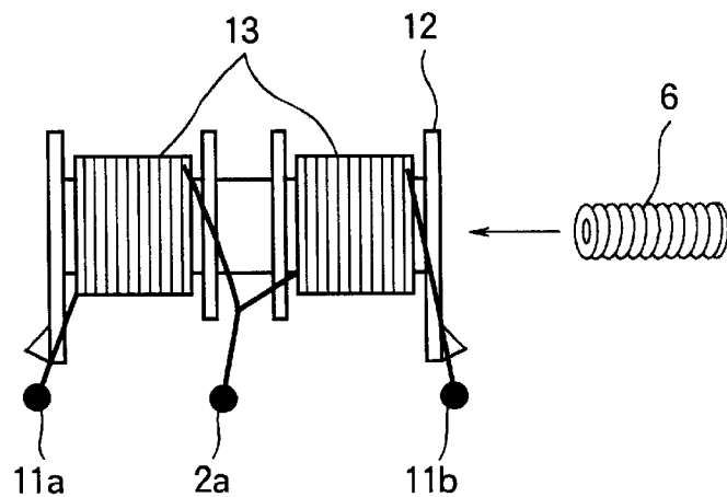
CONVENTIONAL ART
