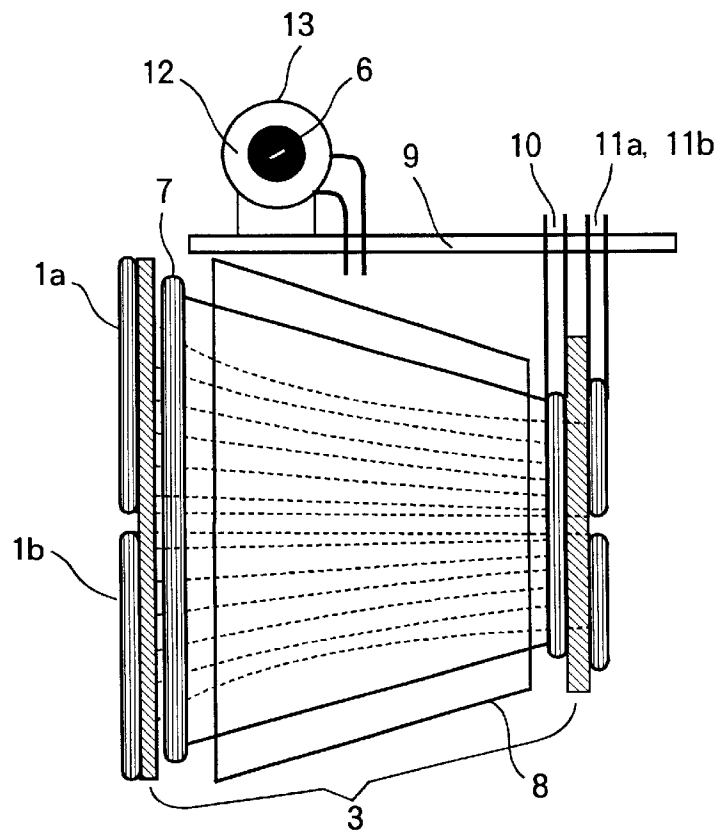
CONVENTIONAL ART
