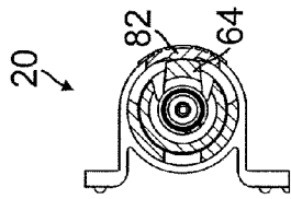
FIG. 2 SECTION C-C
