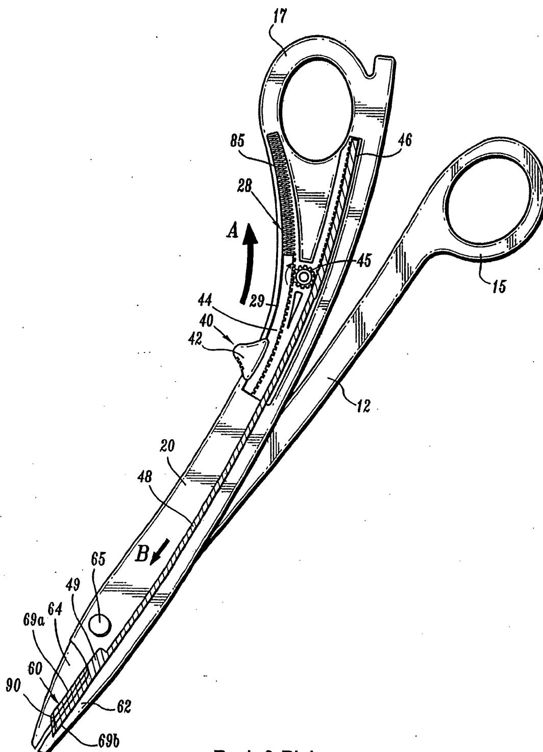
Rack & Pinion FIG. 1C
