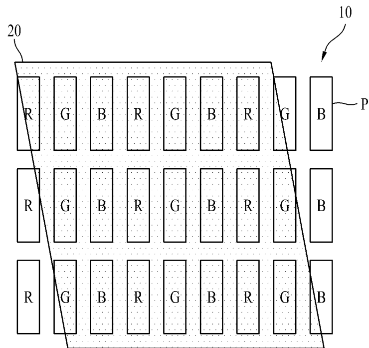
FIG. 1 (RELATED ART)
