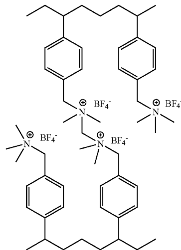
Scheme 5 - Structure of crosslinked P[VBTPMA][BF4]
