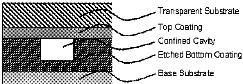
(b) Example fluidic chip configuration with top & bottom etched coating #2
