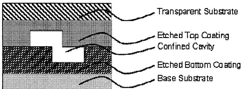
(c) Example fluidic chip configuration with top & bottom etched coating #3
