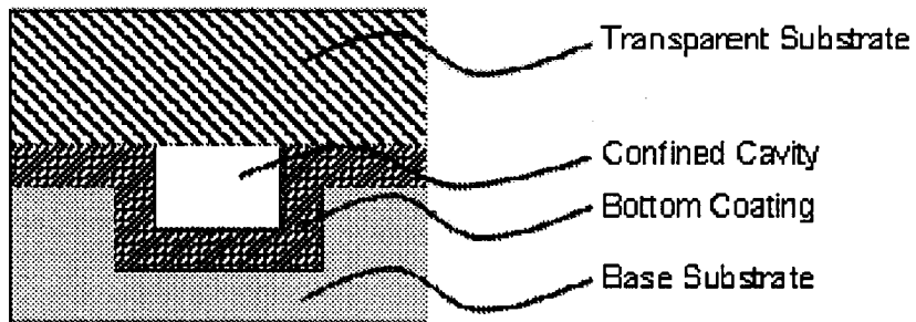
(b) Example fluidic chip configuration with bottom coating #2
