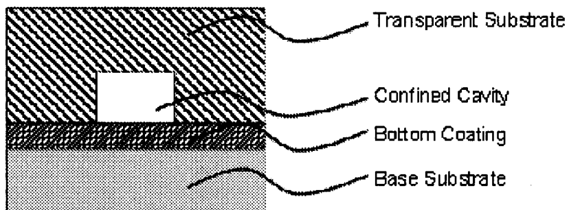
(c) Example fluidic chip configuration with bottom coating #3
