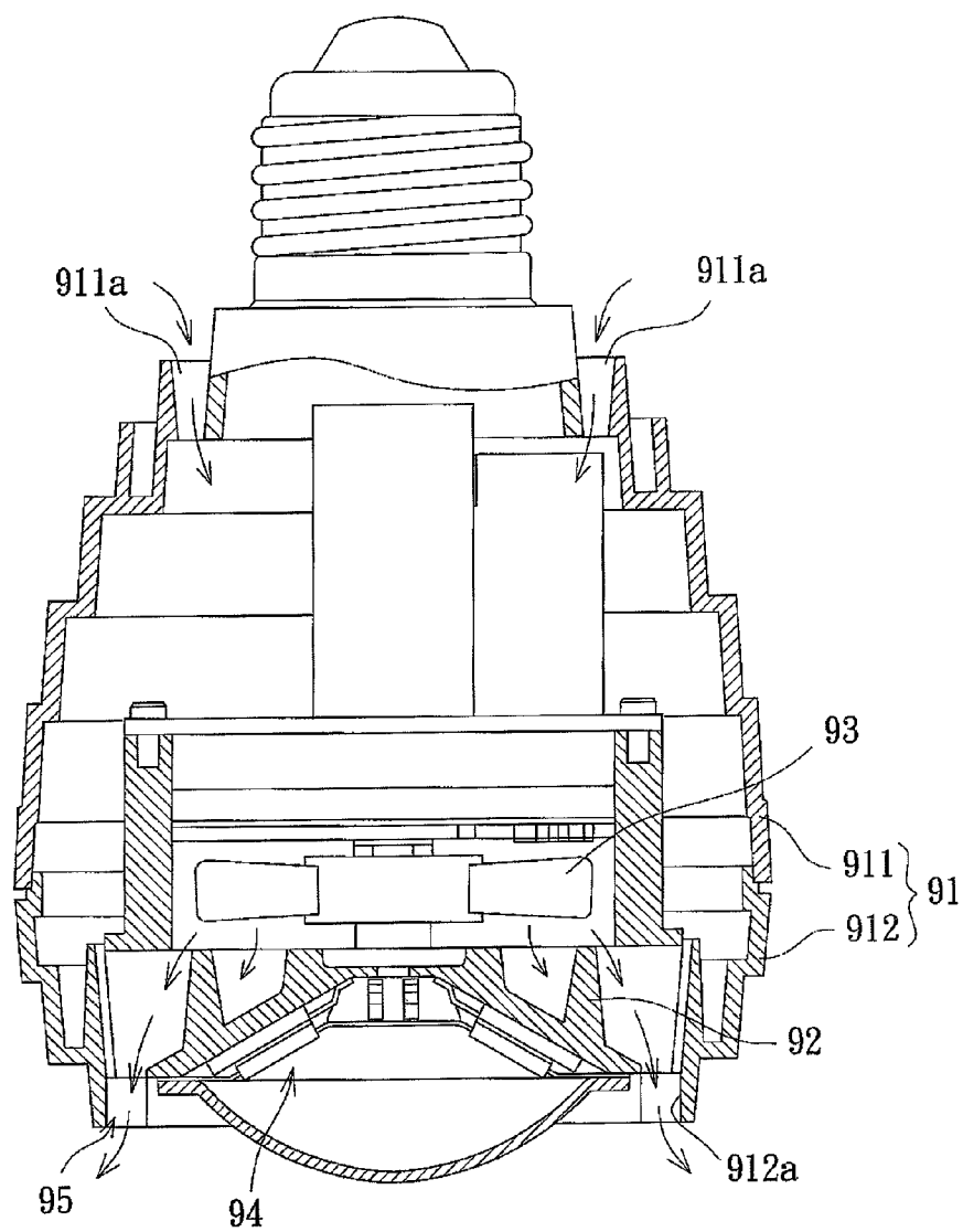
FIG. 2 PRIOR ART
