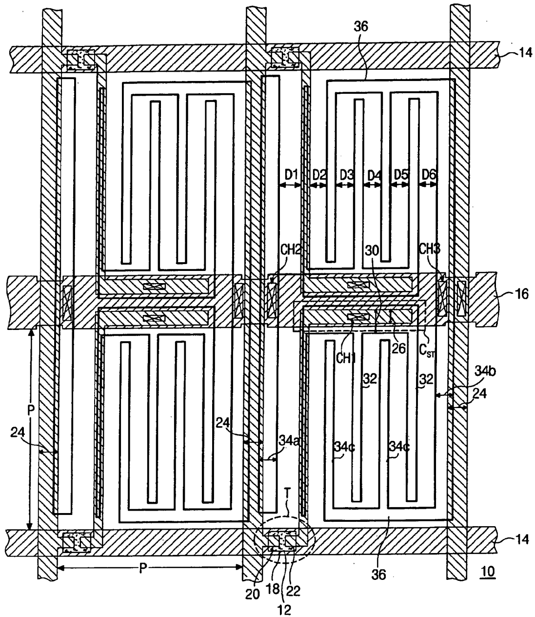
FIG. 2 (RELATED ART)
