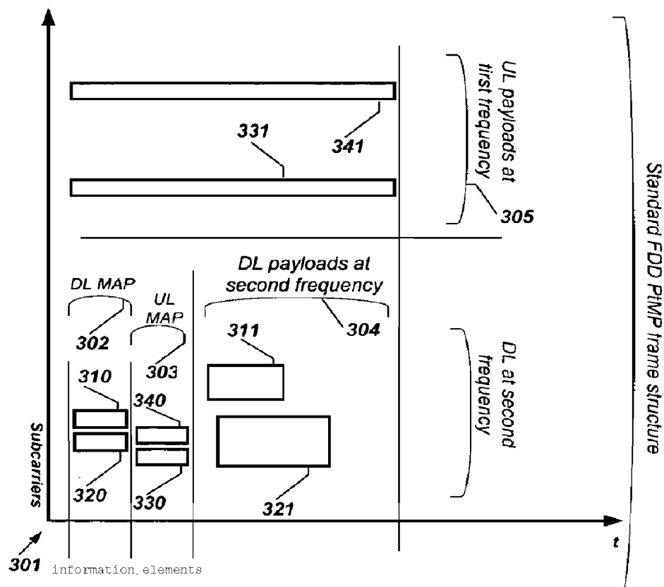
FIG. 4C - PRIOR ART
