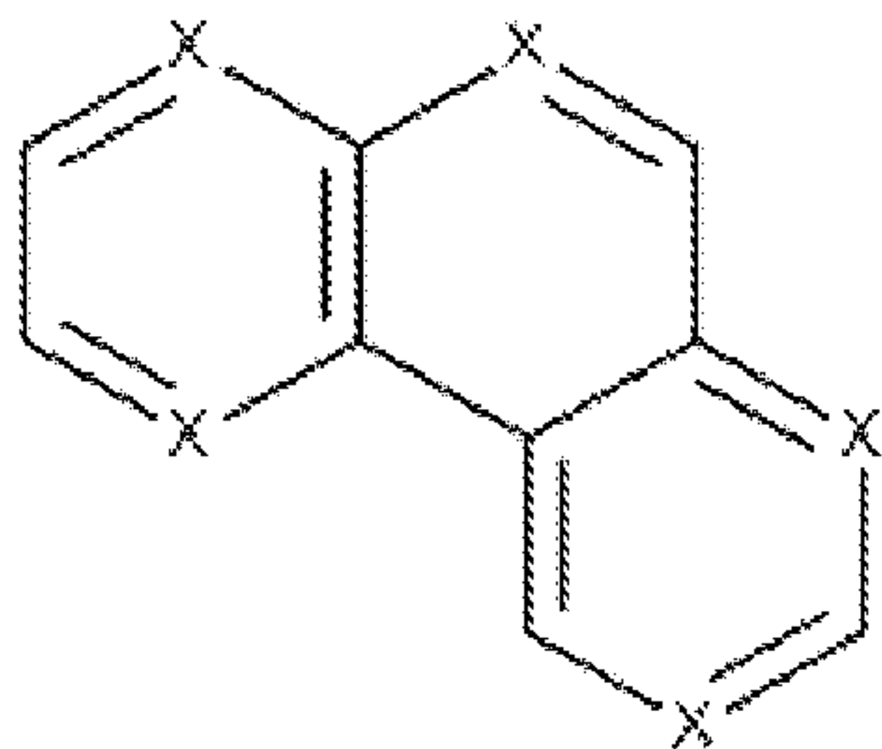
Formula VI
