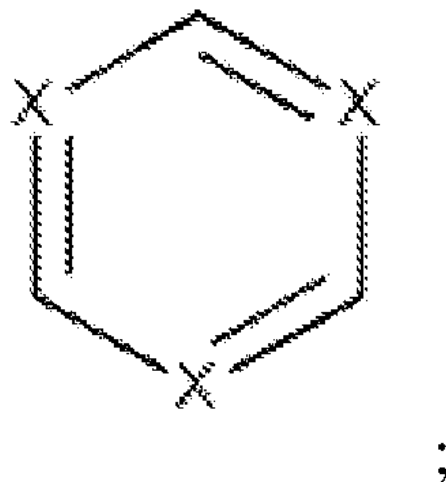
Formula III
