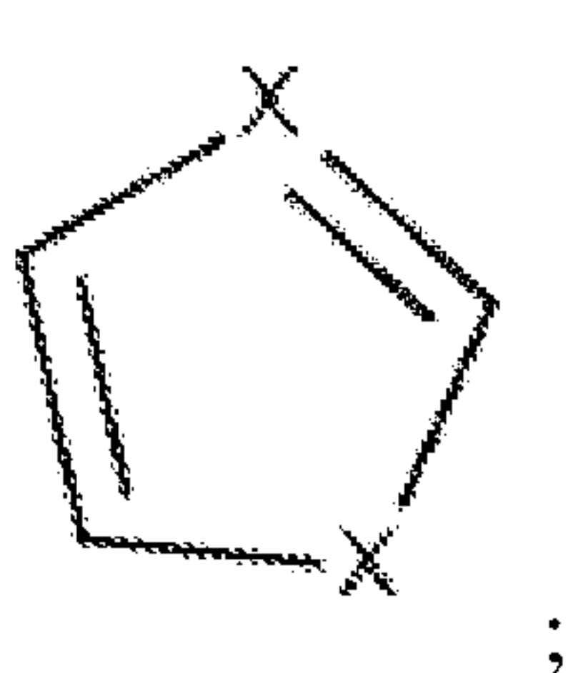
Formula II
