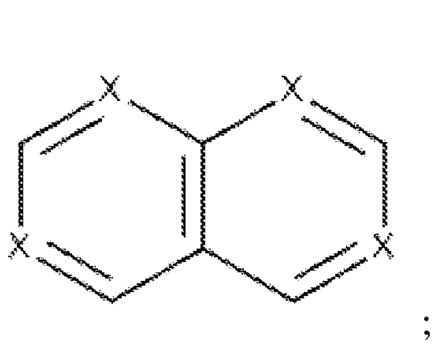
Formula VI
