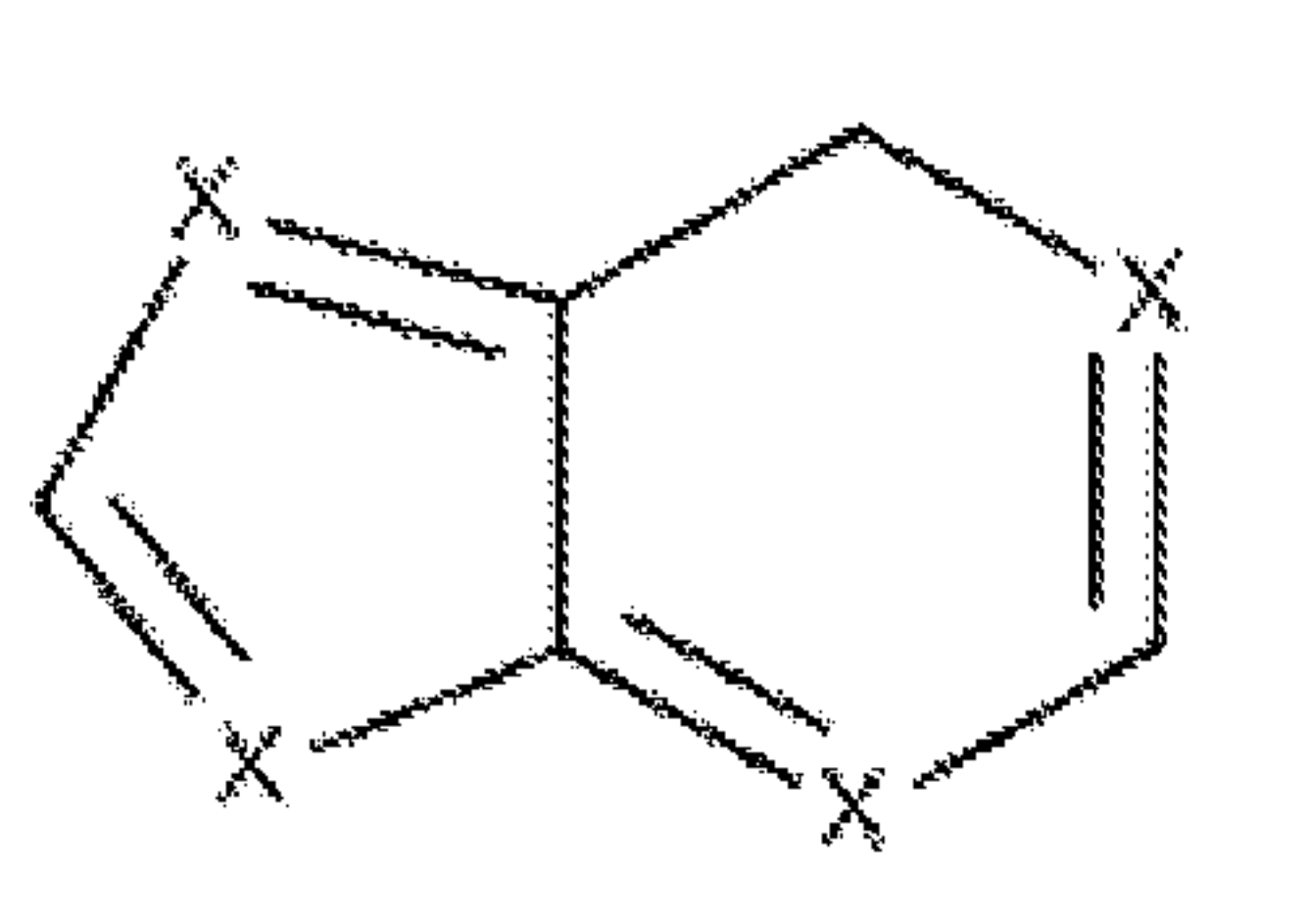
Formula IV
