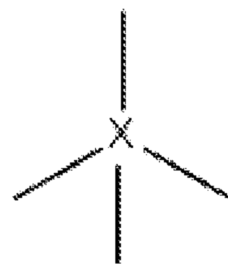
Formula VII;
