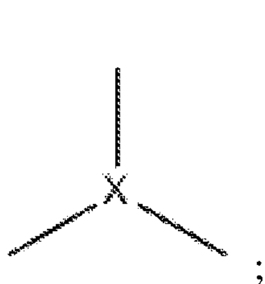
Formula I
