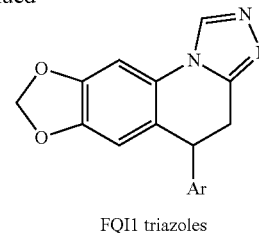
FQI1 triazoles
